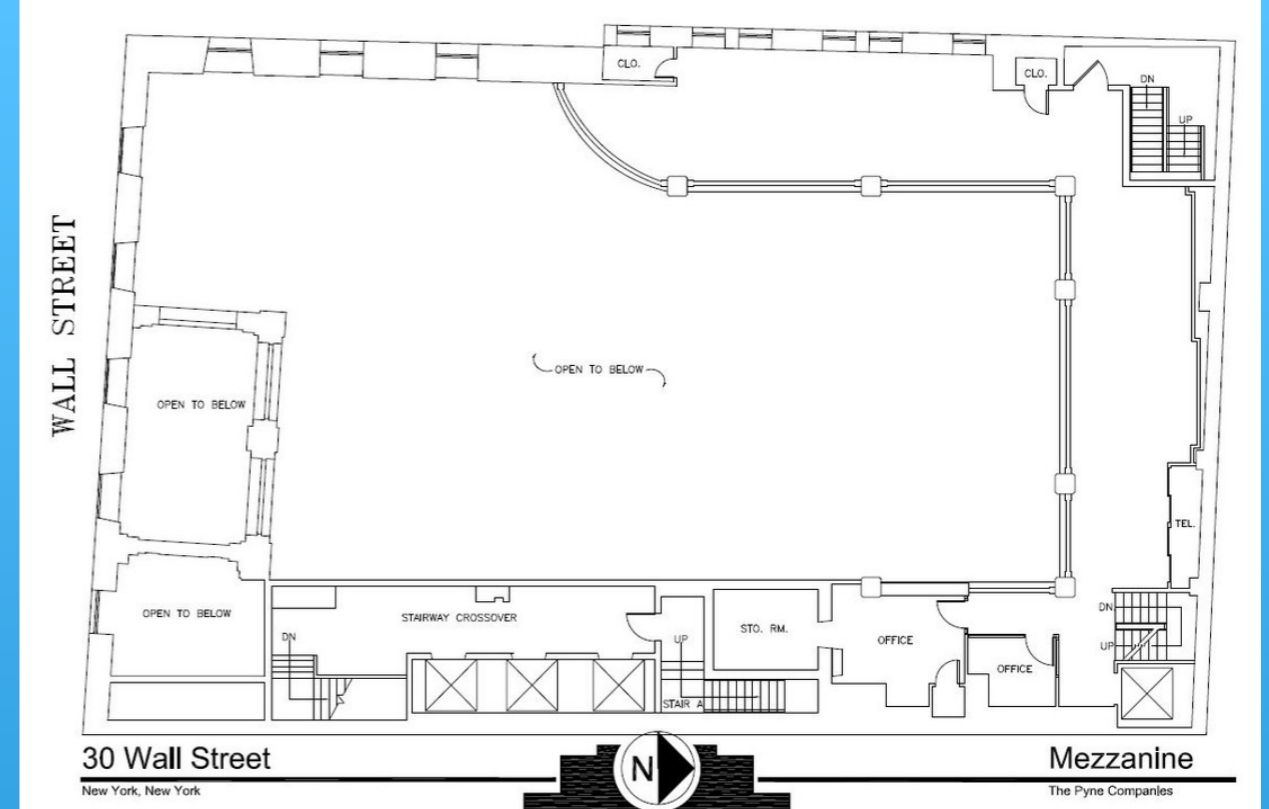
Ground Floor 7,523 sf – 20' Ceilings
